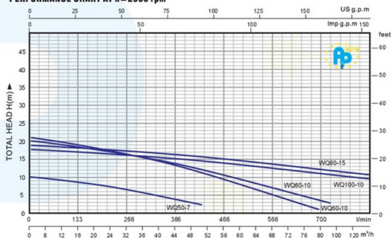
PERFORMANCE CHART AT n=2900 rpm
