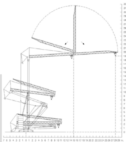
PLUMA HORIZONTAL
